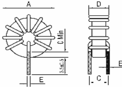
Figure 1 (standard type)
