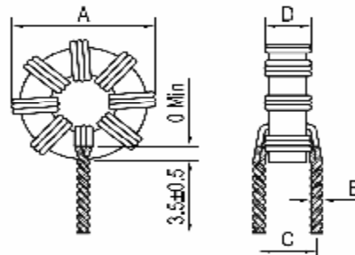
Figure 2 (multiwire type)
